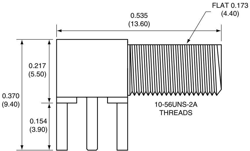
SIDE VIEW
