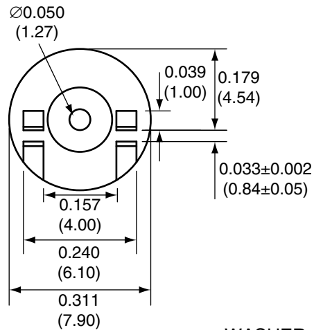
WASHER
