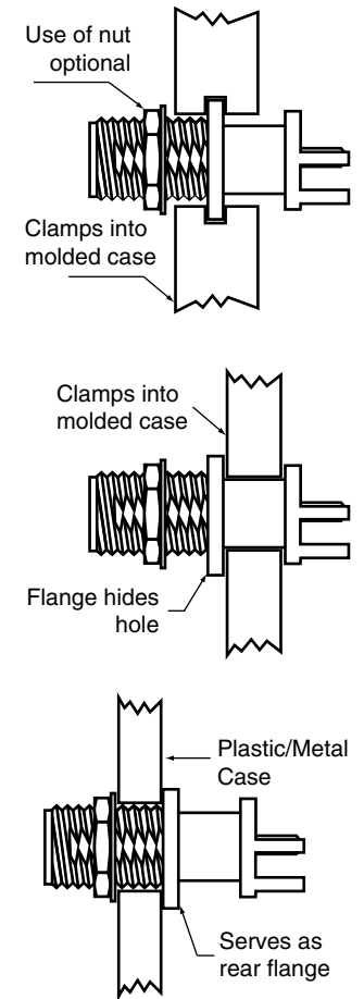
MOUNTING METHODS
